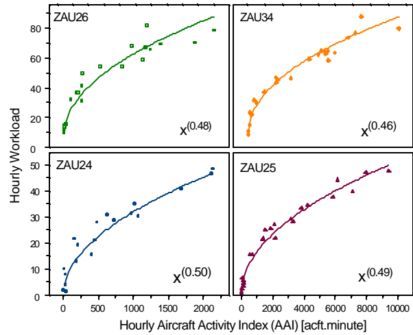
FIGURE 12. Power regression for the Aircraft Activity Index (AAI) vs. Workload for sample sectors in the ZAU Center.
